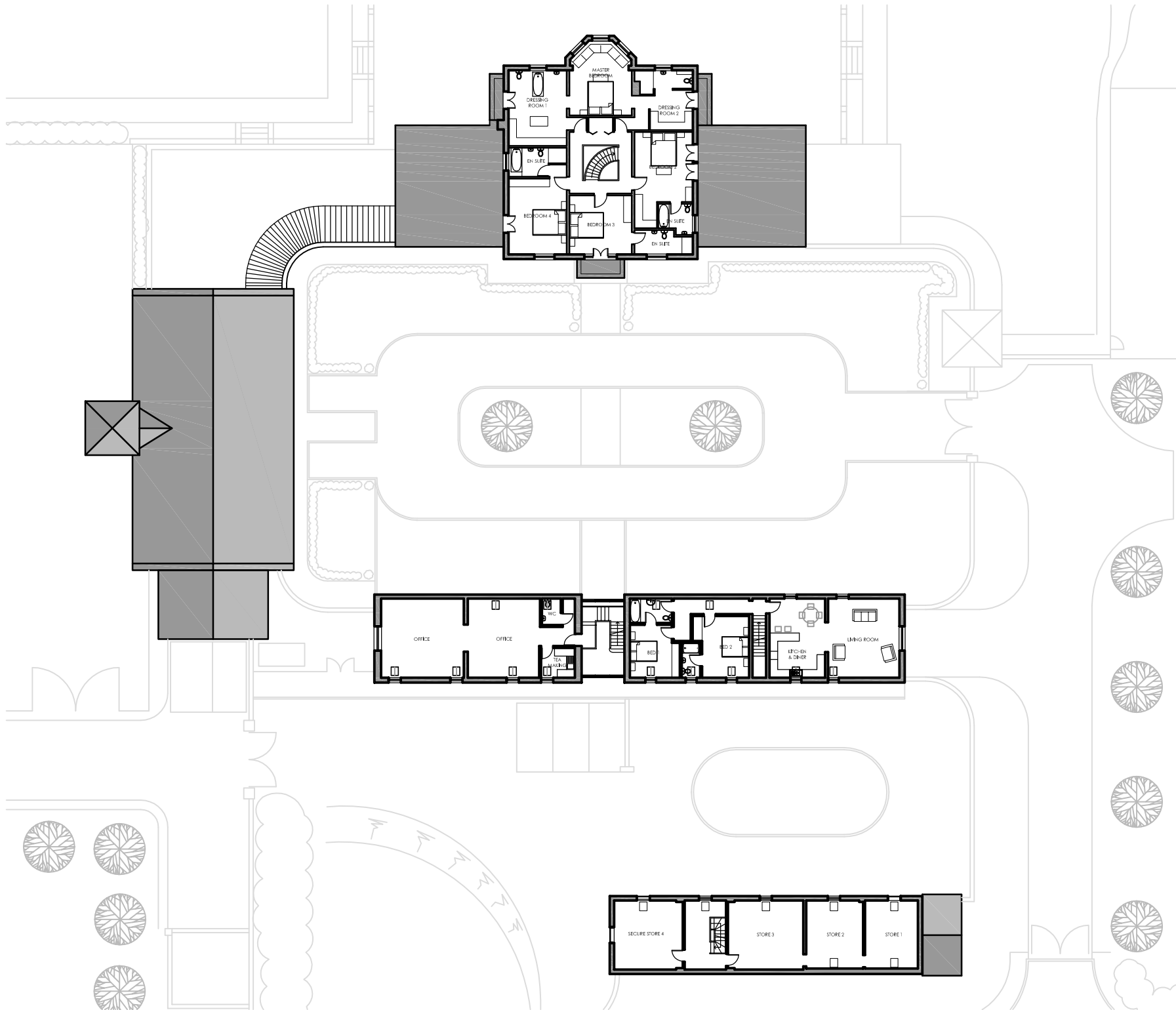
Chidlow Hall First Floor Plan
