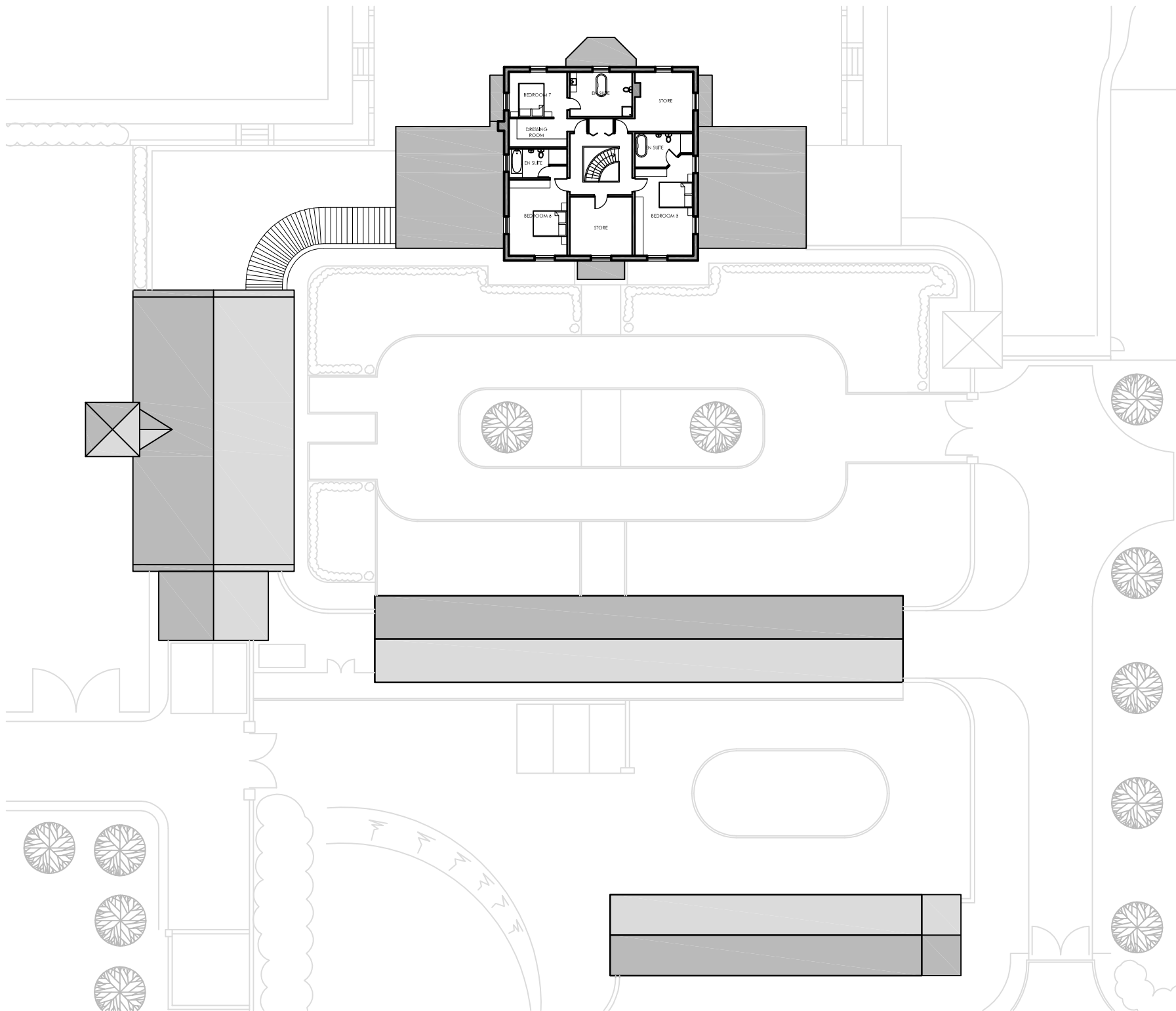
Chidlow Hall Second Floor Plan
